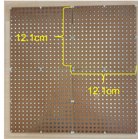
28 GHz RIS prototype
