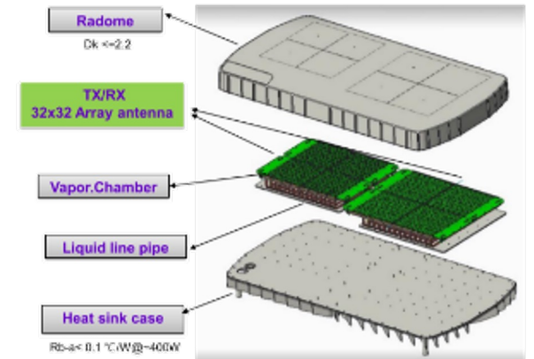
Ku-band LEO User Terminal
